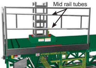
Door support guardrail
