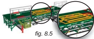
fig. 8.5 Temporarily store sliding doors on the deck of the unit
