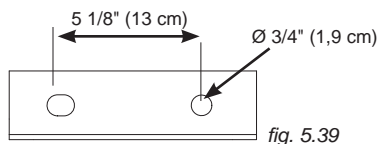
fig. 5.39 Wall tie bracket template
