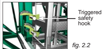
fig. 2.2 Safety hooks in emergency activation position
